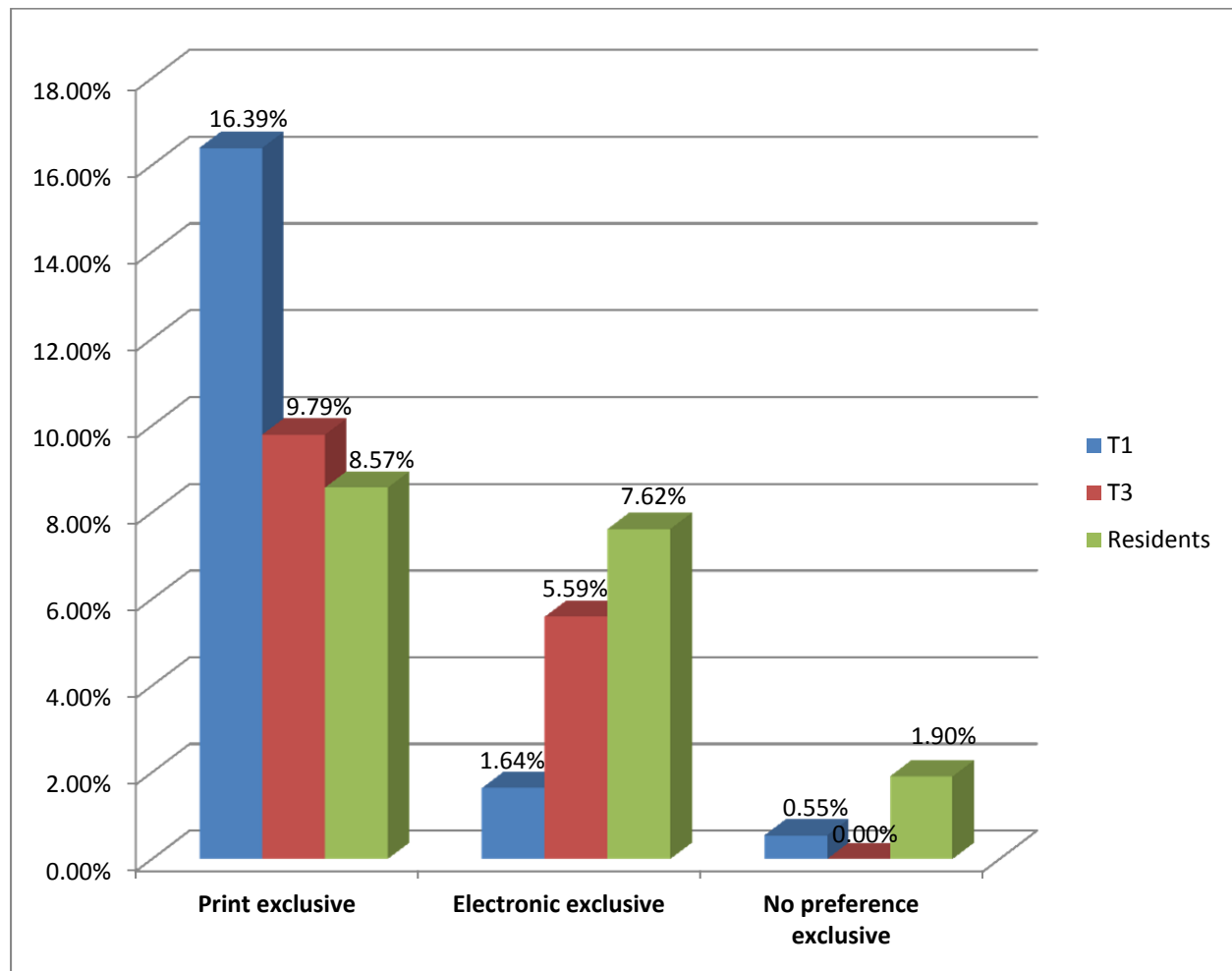
Figure 6 Exclusive preferences
